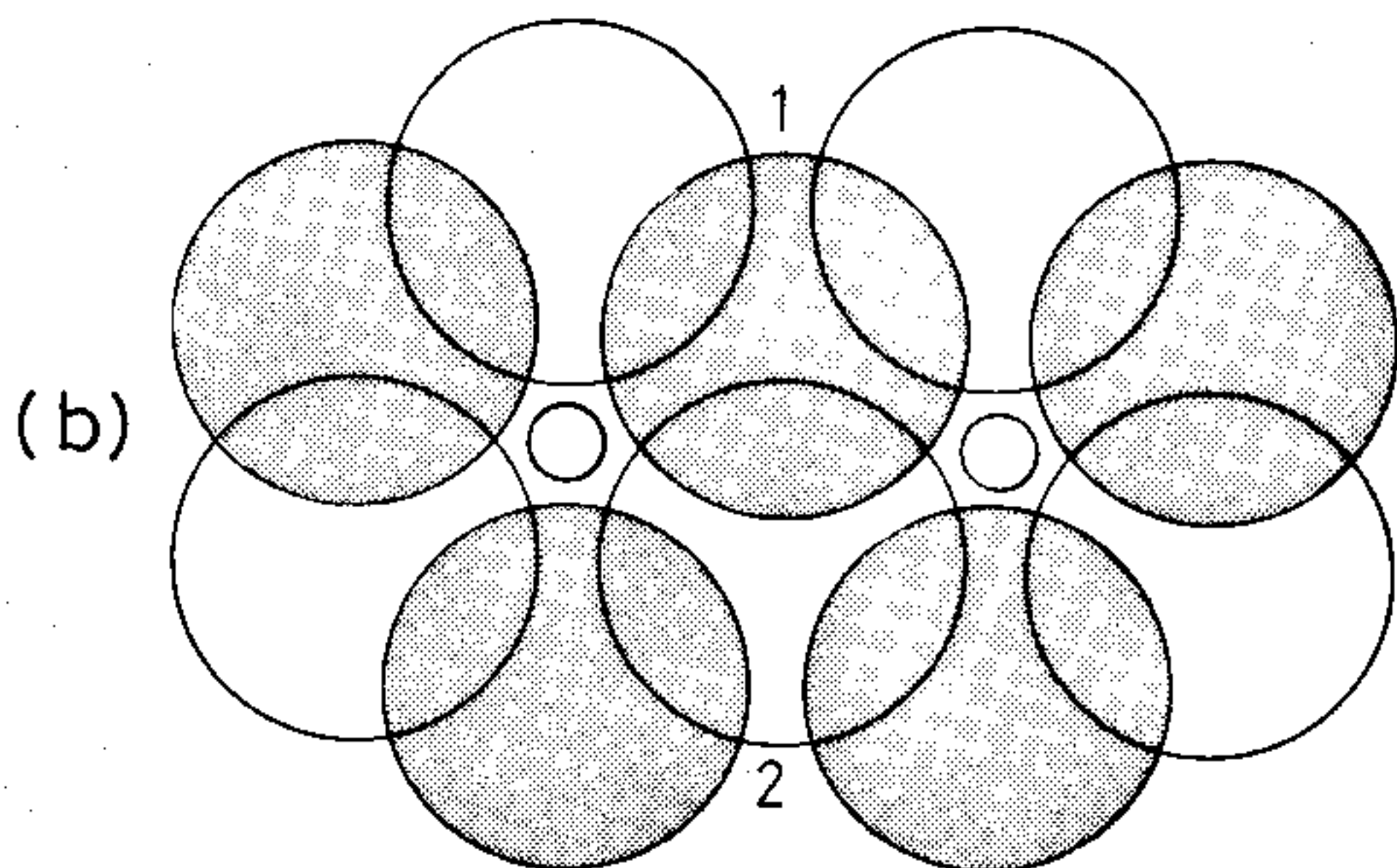
Fig. 7.21 The rutile structure: (a) in idealized form, with planar oxide layers; (b) edge-sharing octahedra
