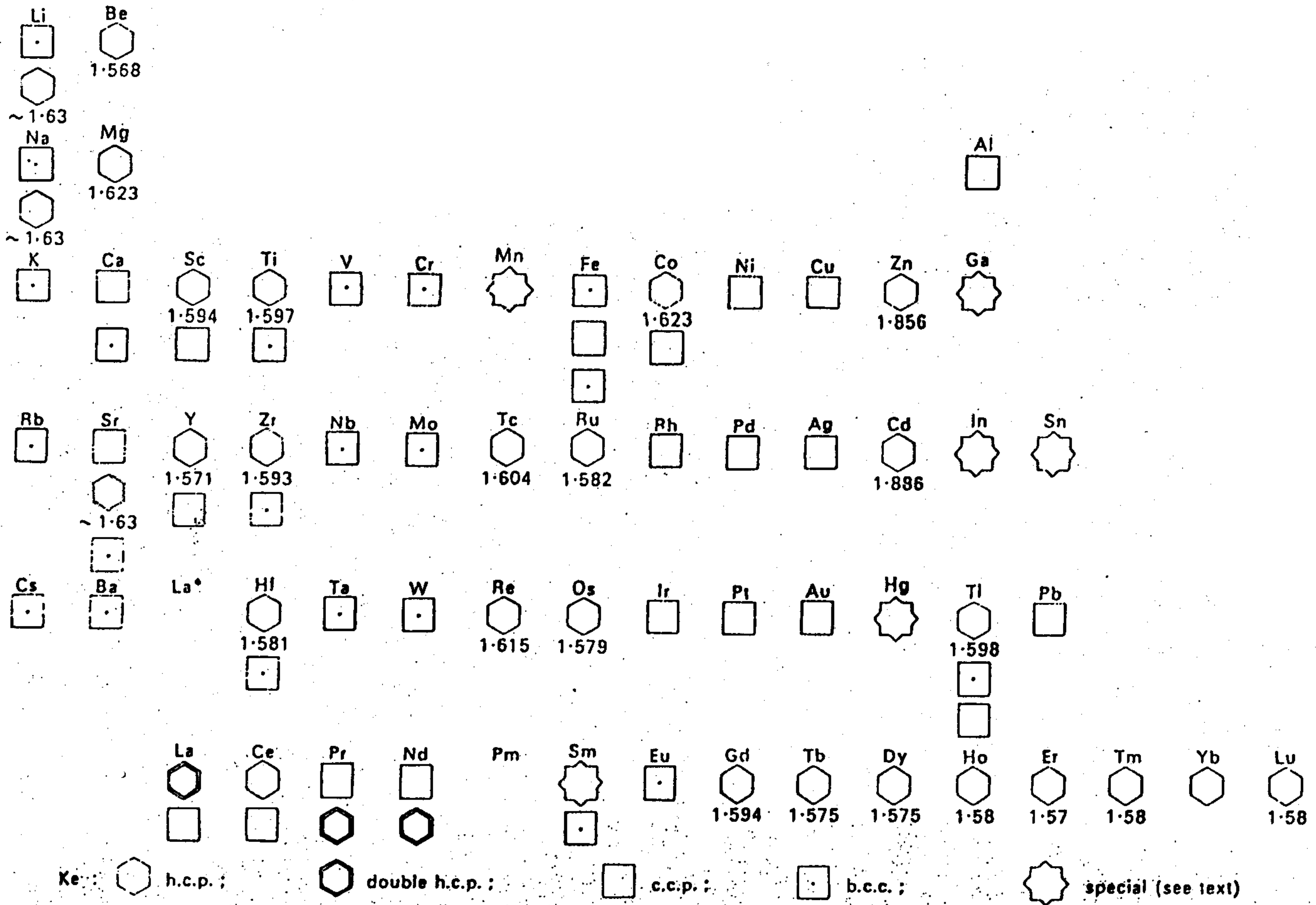
Figure 8-1 Structures of the metallic elements. Where more than one structure is adopted by an element, the most stable form is given first and less stable ones underneath. For hexagonal structures the c/a ratio is also given
